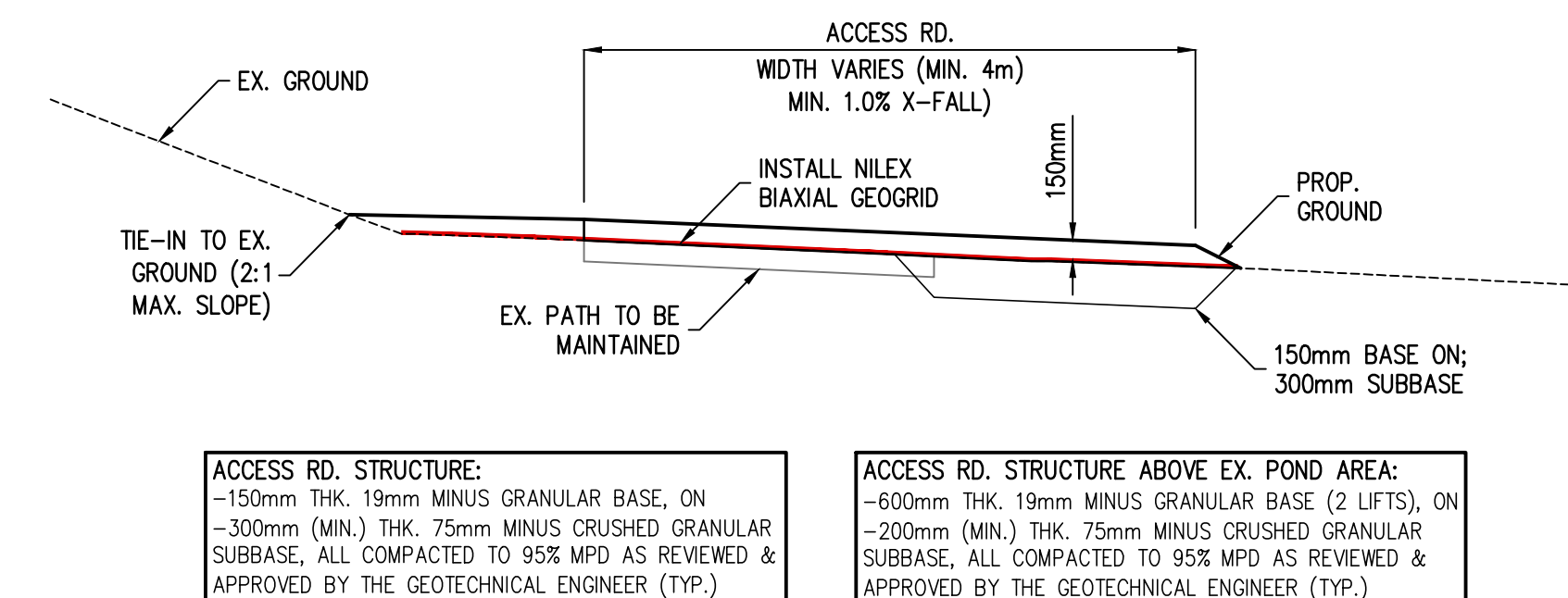
CRANE ACCESS ROAD TYPICAL SECTION SCALE 1:50
