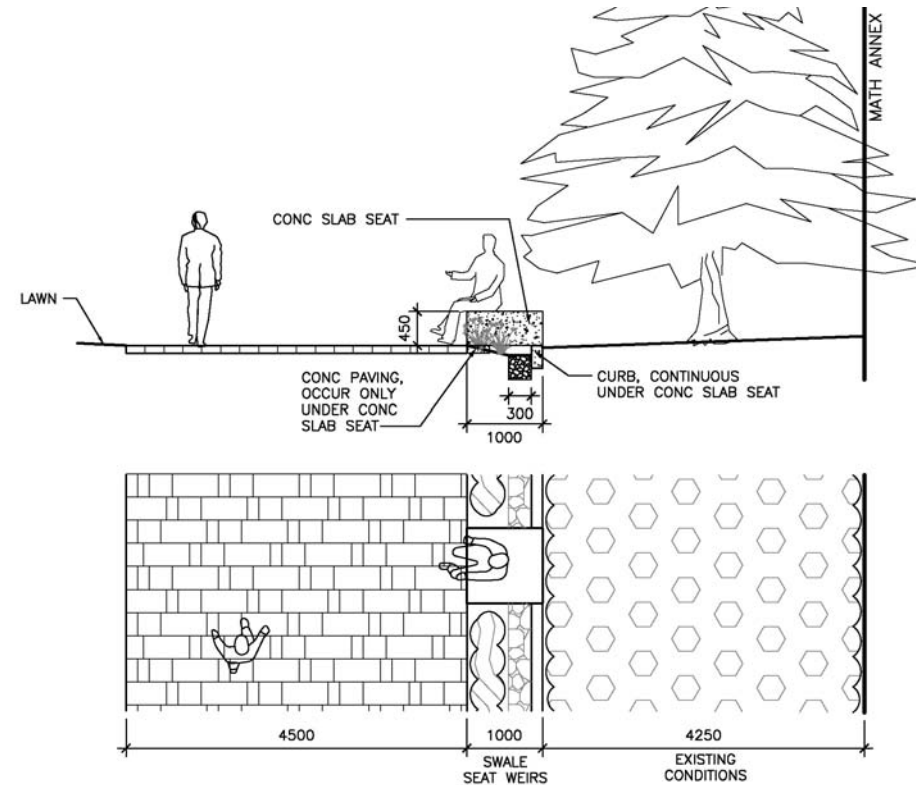
RUNNEL PLAN / SECTION
