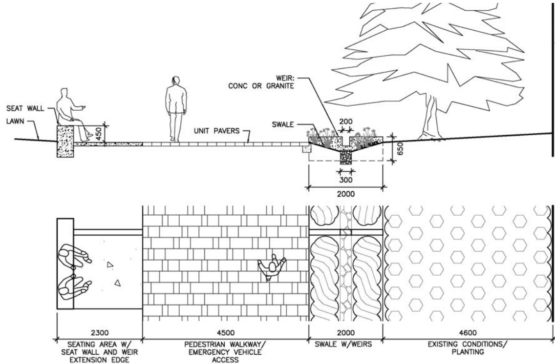
WEIR & SWALE PLAN / SECTION
