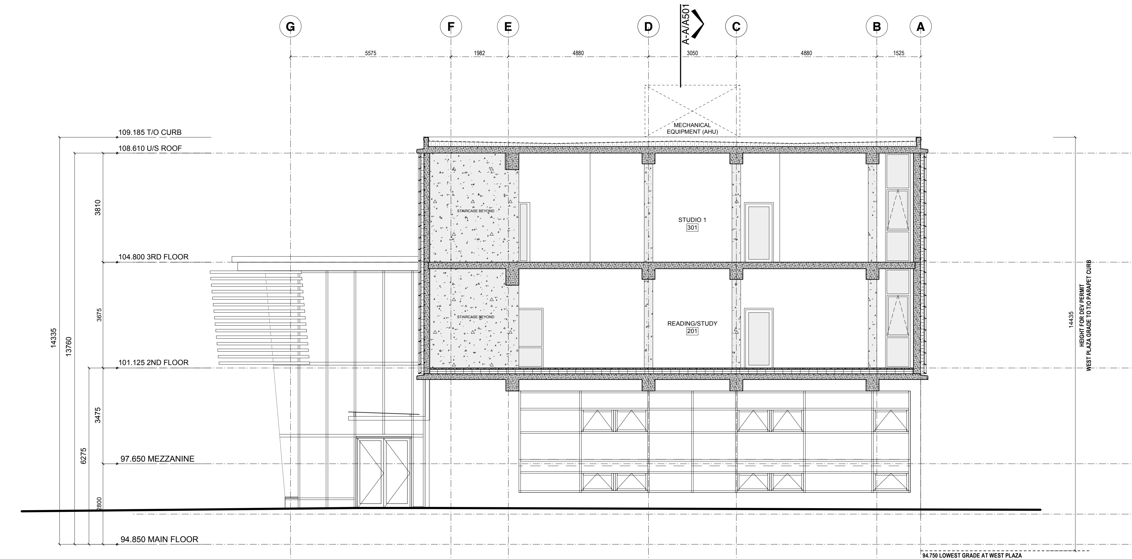
SECTION C-C
