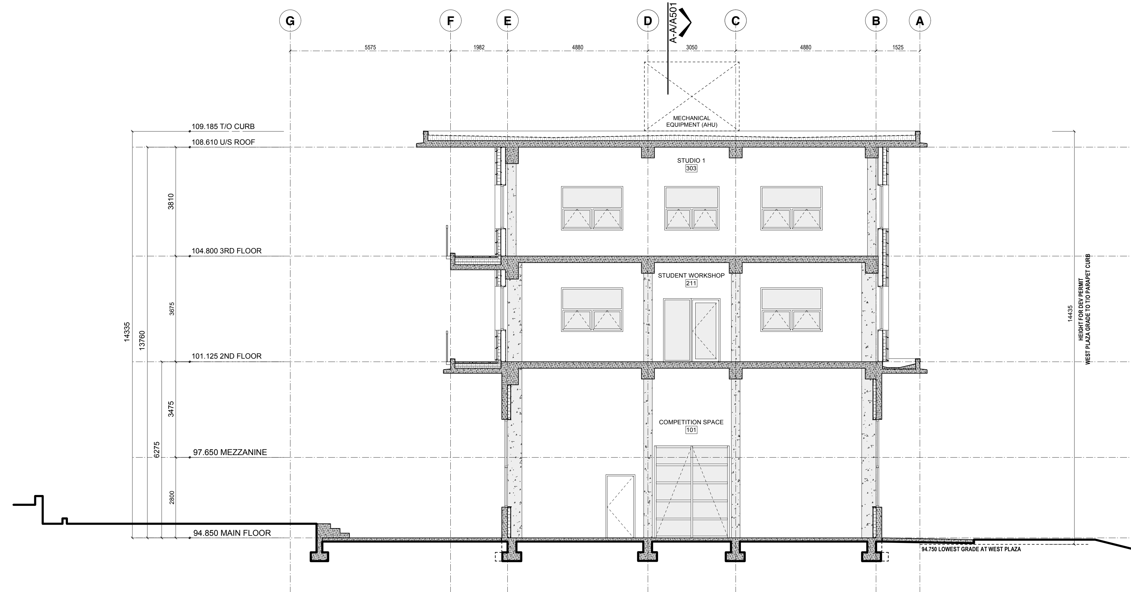
SECTION C-C
