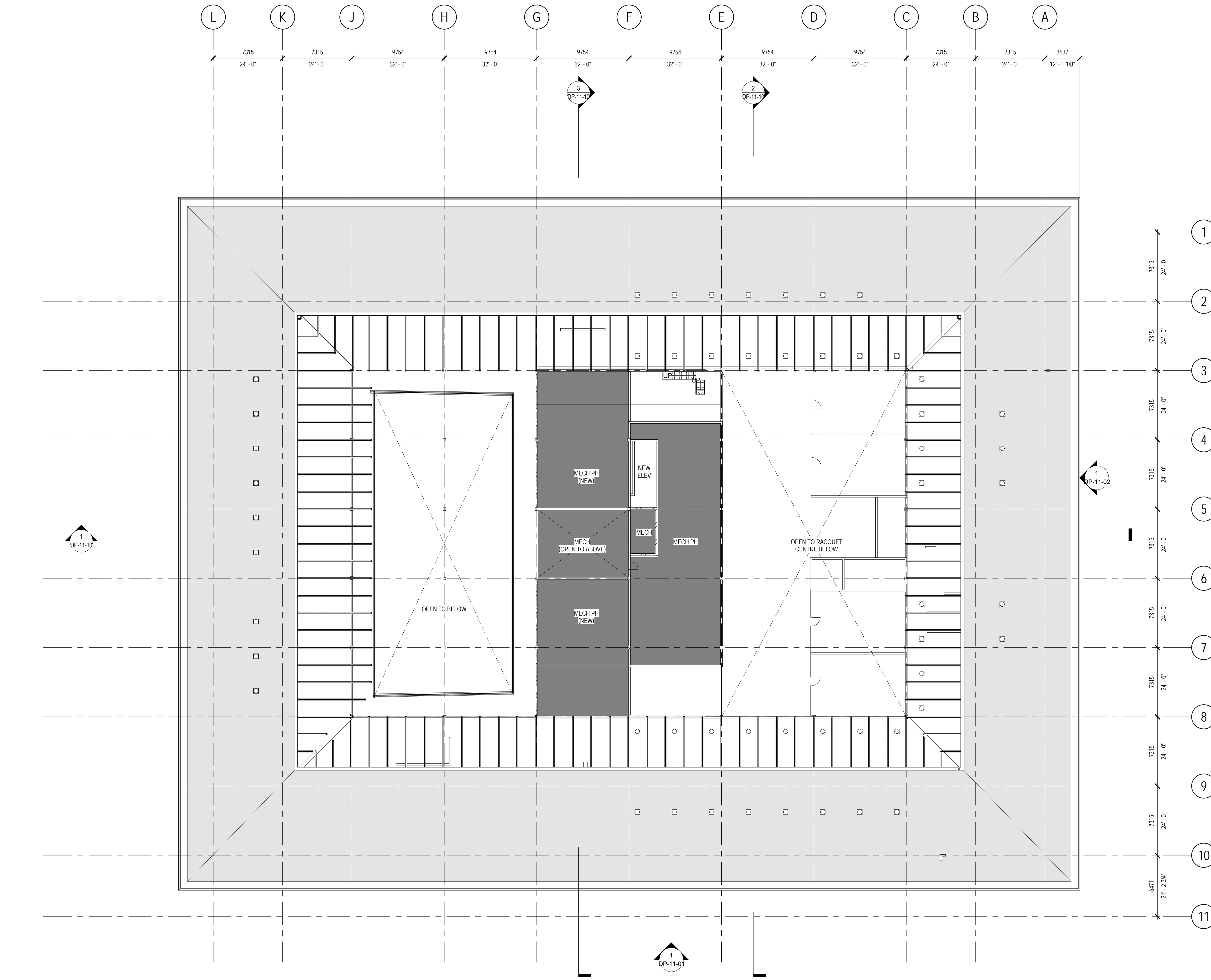
1 FLOOR PLAN - MECH PENTHOUSE 1: 200
