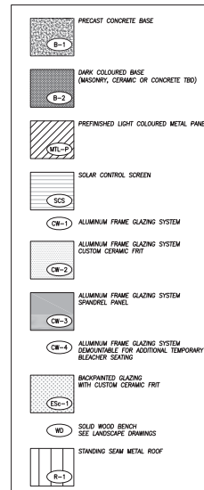
5 EXTERIOR ELEVATION MATERIAL KEY 1:100
