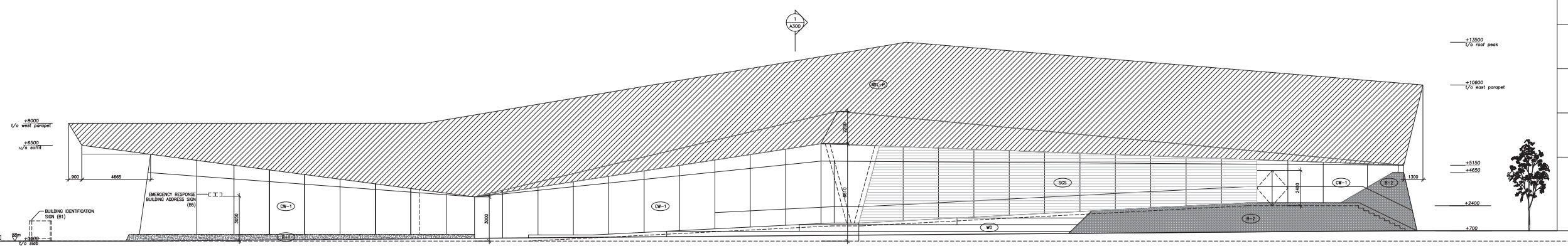
2 SOUTH ELEVATION 1:100
