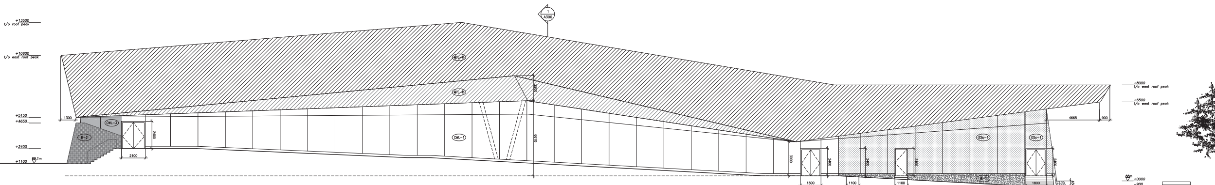
1 NORTH ELEVATION 1:100
