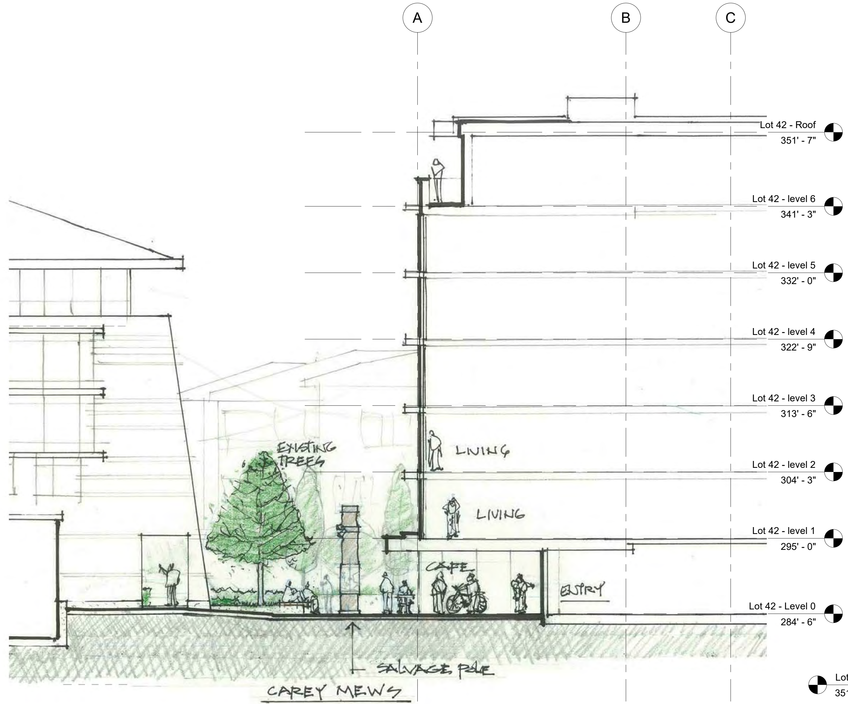
1 Landscape Section - Mews 1/8" = 1'-0"
