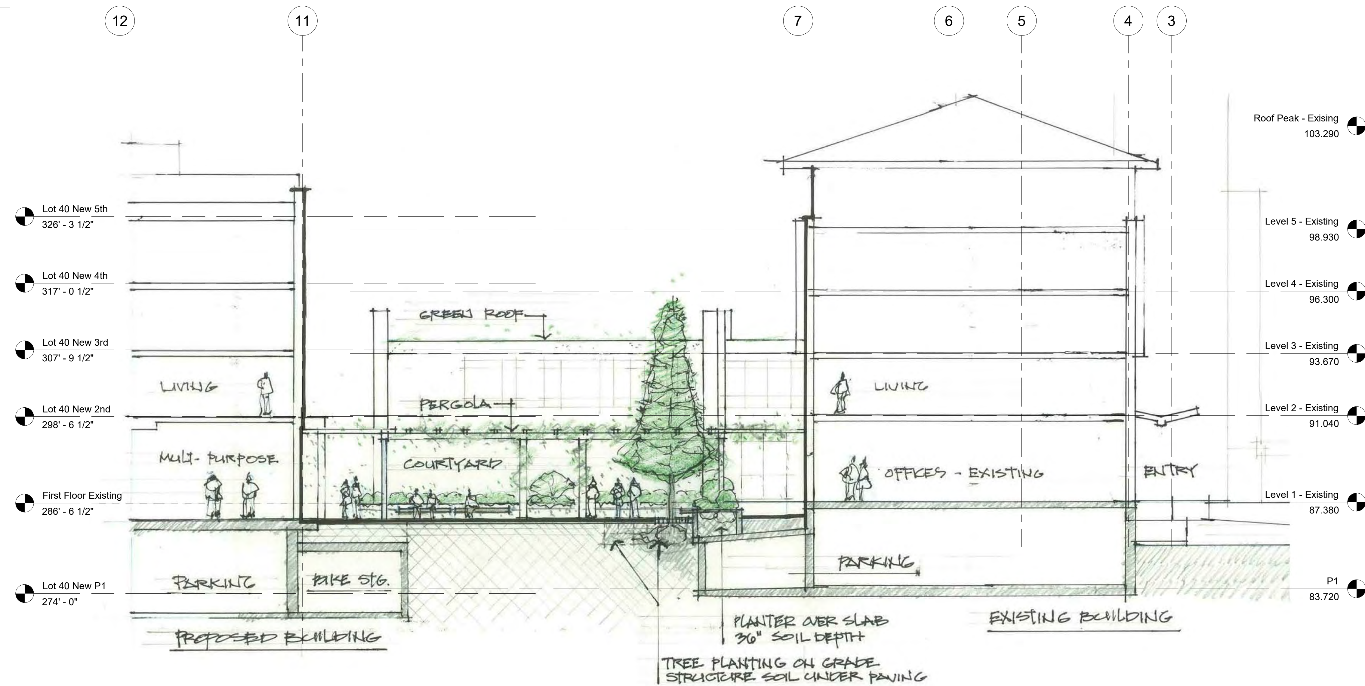
2 Landscape Section - Courtyard 1/8" = 1'-0"
