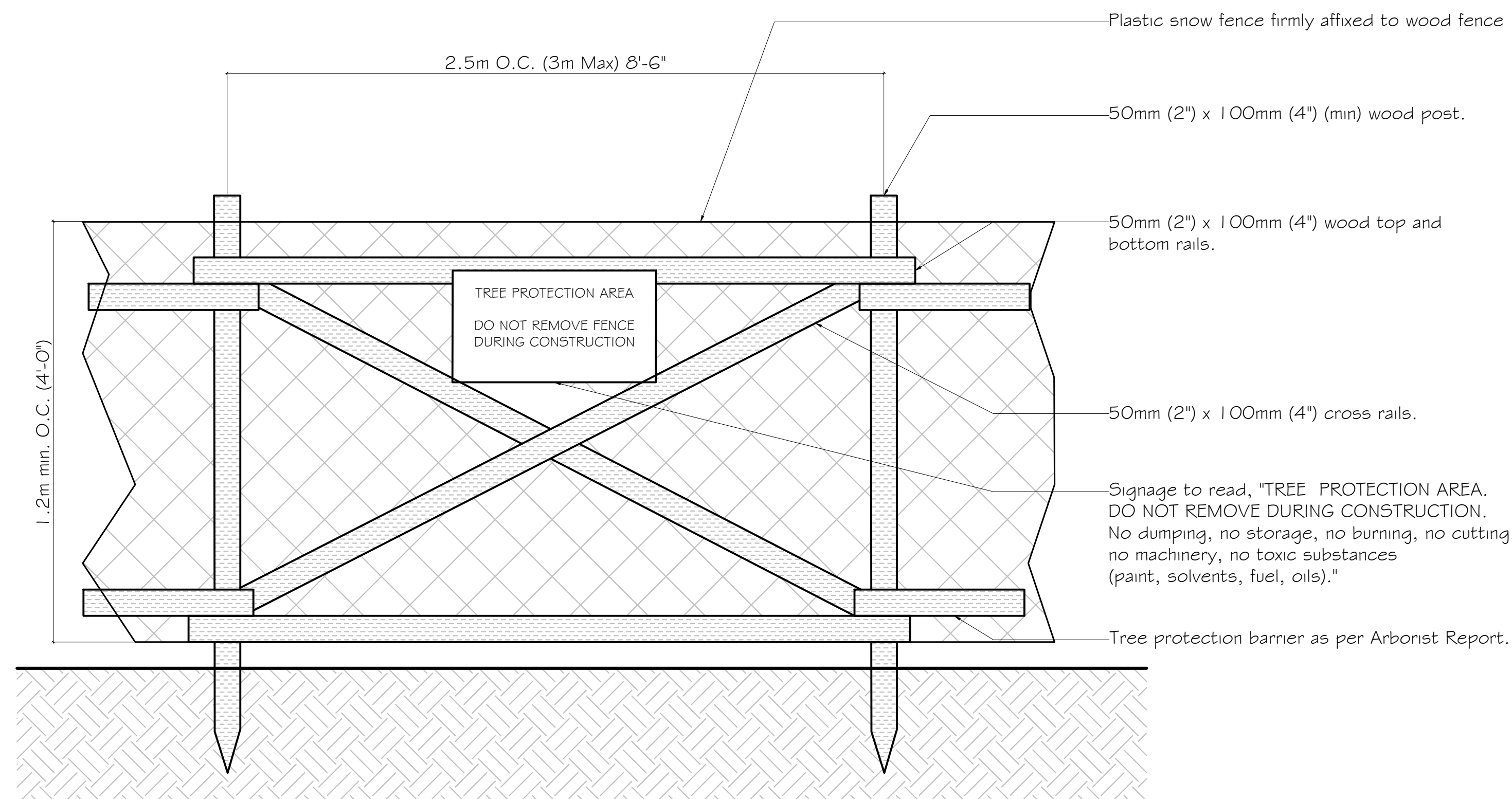
6 Typical Tree Barrier Details 3/4" = 1'-0"
