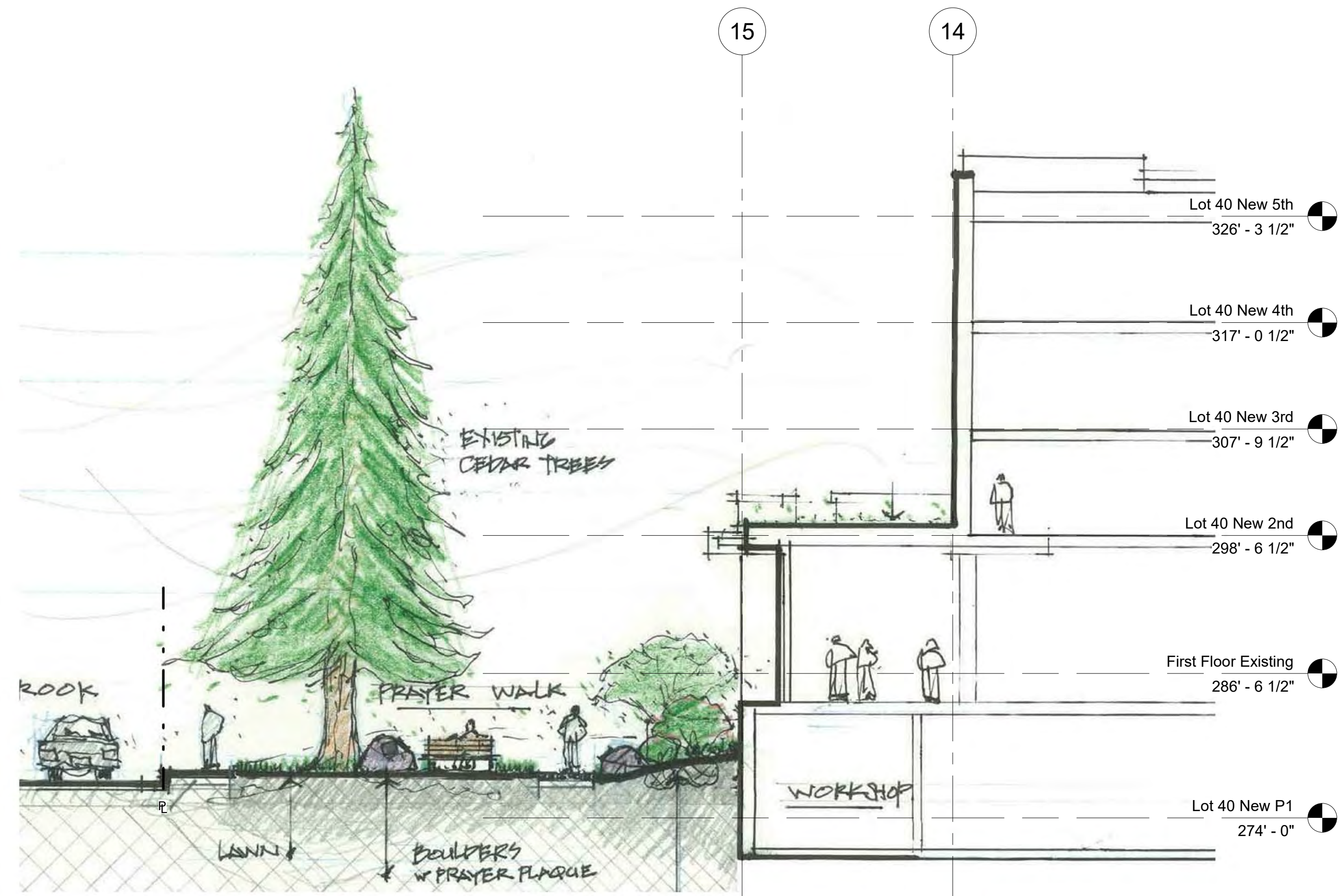
1 Landscape Section - Wesbrook 1/8" = 1'-0"
