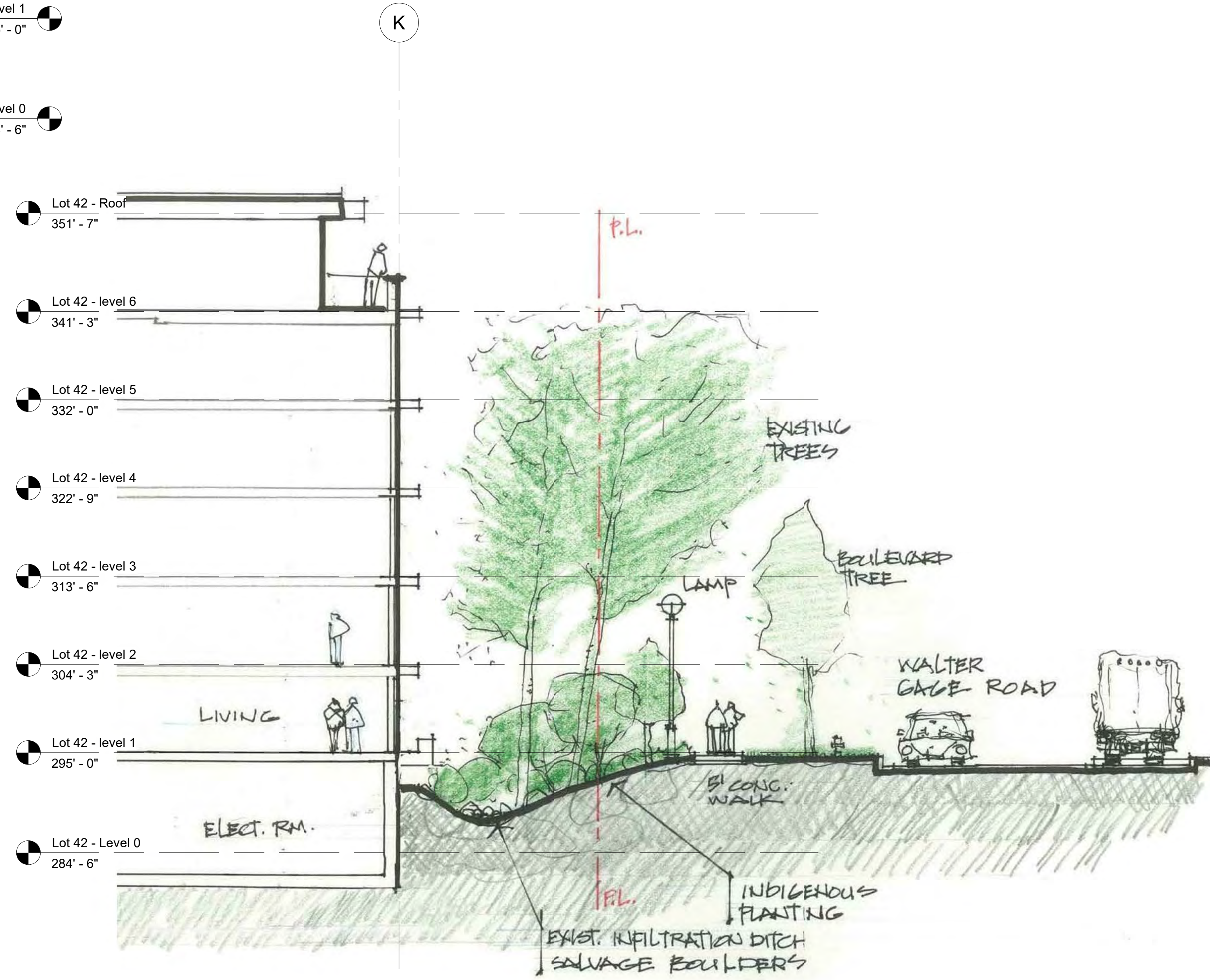
2 Landscape Section - Gage 1/8" = 1'-0"
