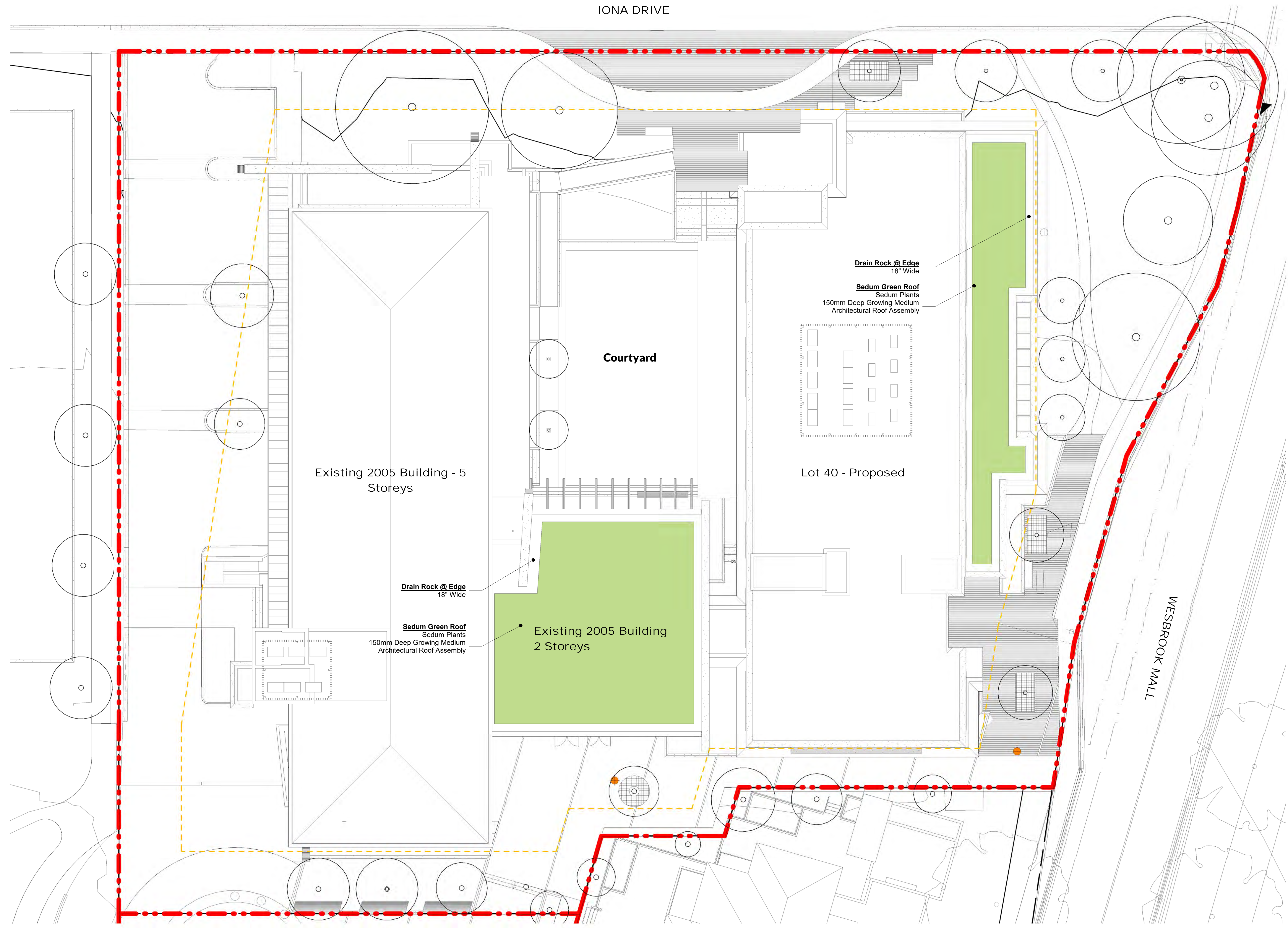
1 Planting Roof - North 3/32" = 1'-0"
