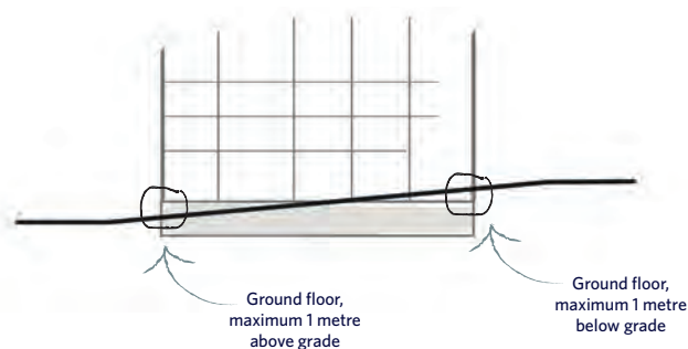
Figure 38. Allowable residential ground floor height from grade
