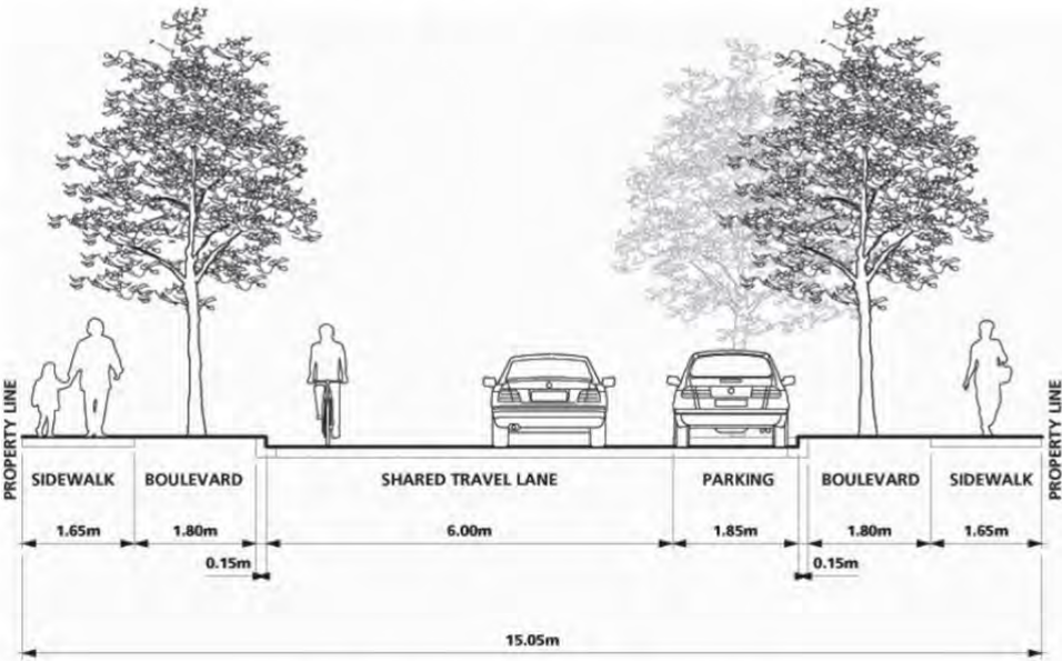
LOCAL STREET ONE SIDE PARKING
