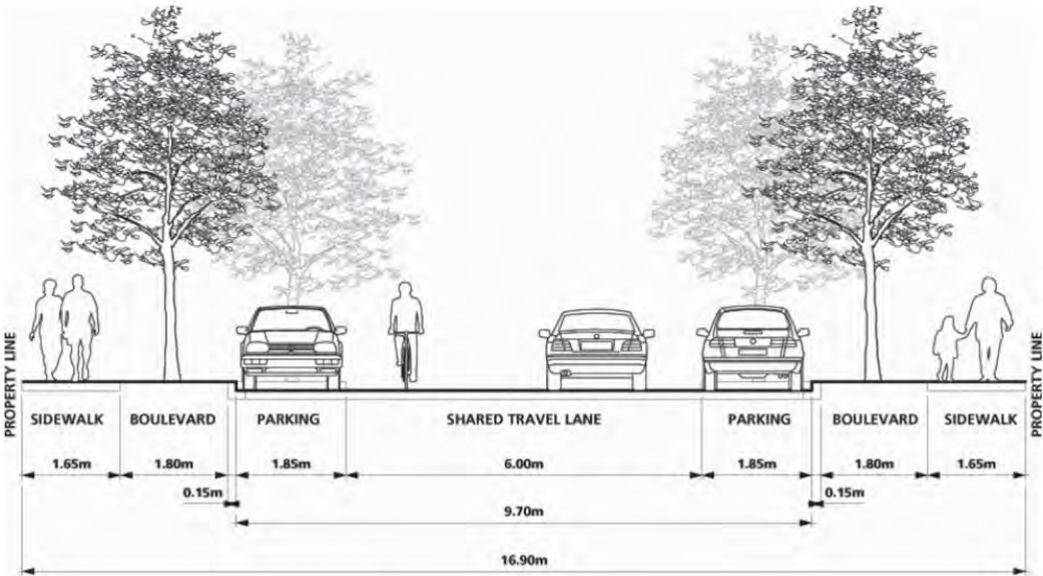
LOCAL STREET TWO SIDE PARKING
