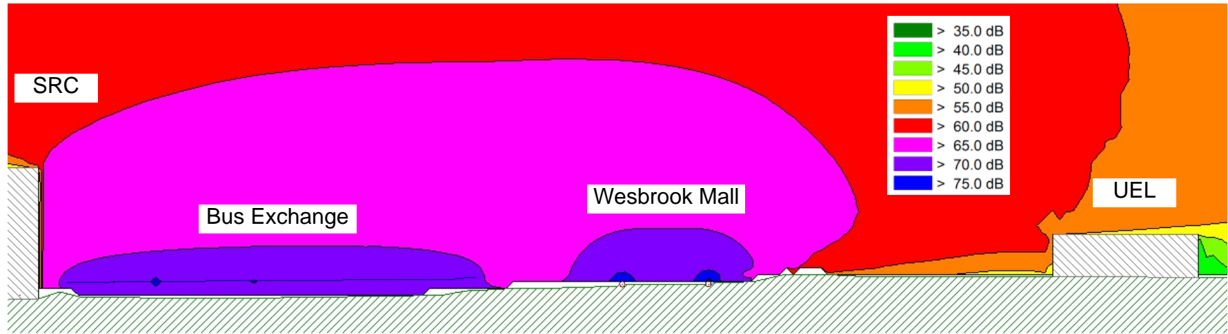
Figure 1: Baseline Cross Section - Daytime Average Noise Prediction through SRC to UEL
