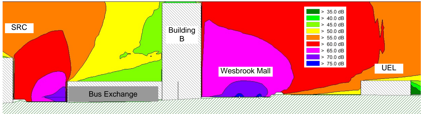
Figure 2: Post-Project Cross Section - Daytime Average Noise Prediction through SRC and Building B to UEL
